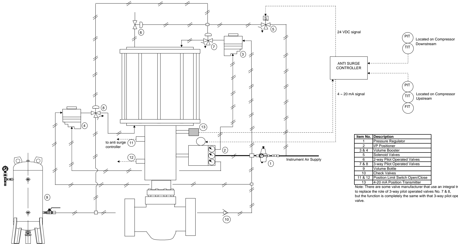
Typical Anti Surge Control Valves General Arrangement
